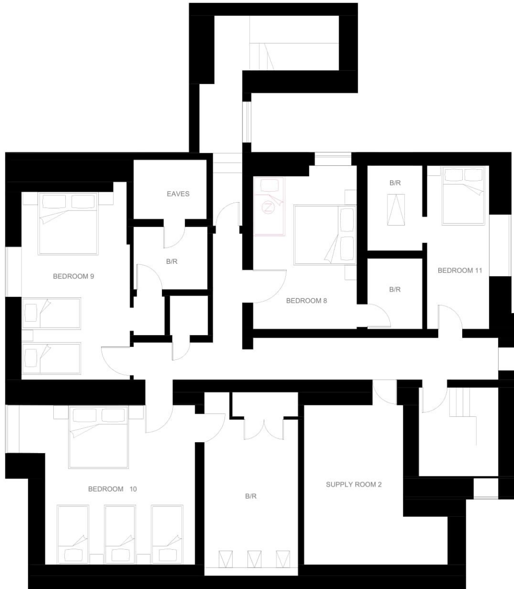
PENCRAIG COURT FLOOR PLAN | SECOND FLOOR
